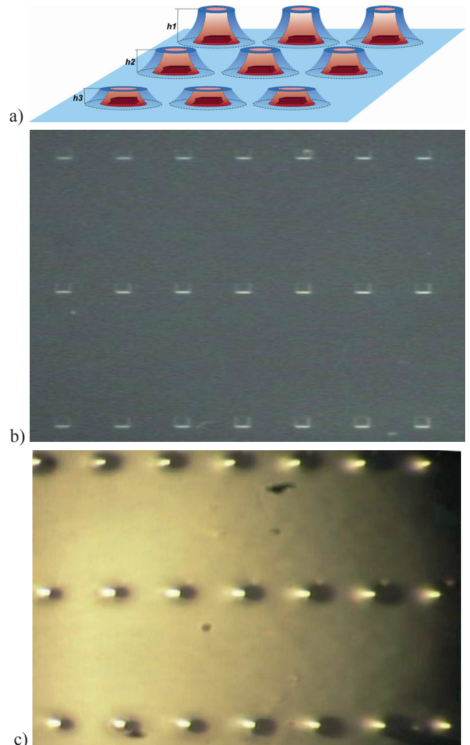
Fig 12. Schematic view of a fragment of 3-color monolithic matrix a); island structures of 80 \times 80 \mu\text{m}^2 dimensions with As implanted surface formed on undoped CdTe substrate b)
