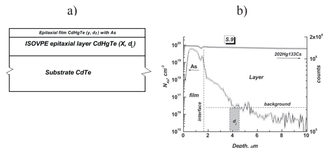
Fig. 4. Scheme of cross section of initial heterostructures S8, S9, S10 (a); SIMS distribution of As and signal of the main component of \text{Cd}_x\text{Hg}_{1-x}\text{Te} solid solution (Hg concentration) in near-surface regions for heteroepitaxial structure of sample S9 (b)
