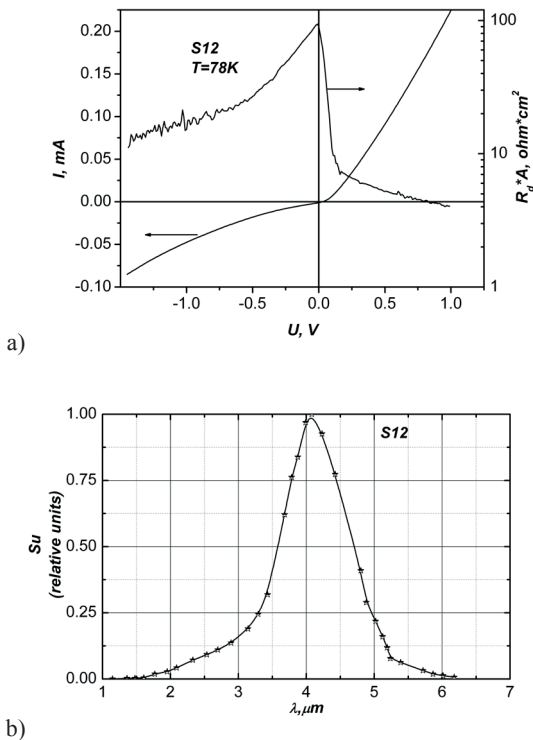
Fig. 8. VAC and dependence of differential resistance normalized by square of voltage for the photodiode obtained in diffusion structure of sample S12 (a). Spectral distribution of photo-signal of photodiode obtained from sample S12 (b)
