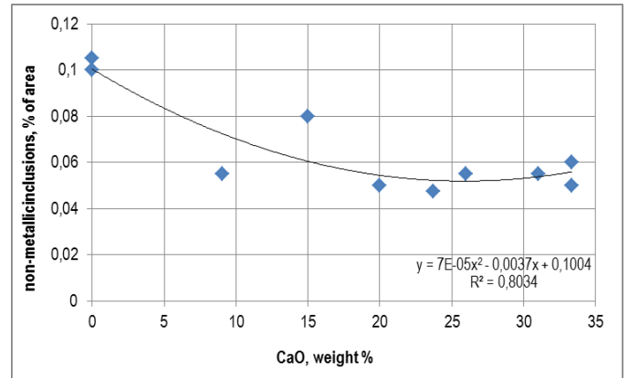
Fig. 4. Impact of the CaO content in the slag on the content of non-metallic inclusions in steel (after ESR)
