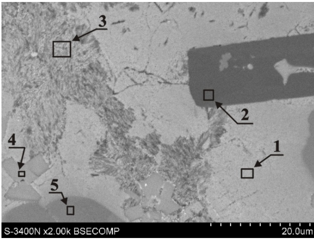
Fig. 6. Microstructure of ZnAl40Cu2Ti alloy after supersaturation and aging 385°C/24 h+150°C/24 h
