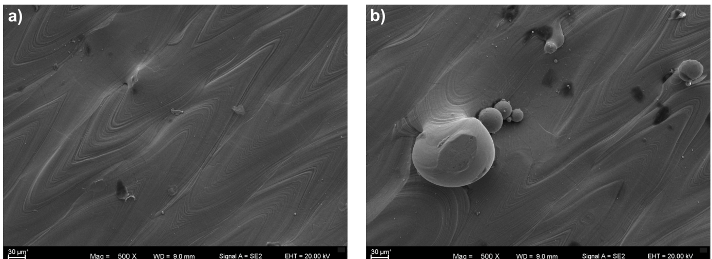
Fig. 2. SEM microphotographs illustrating the morphology of specimens surface after sintering by means of DMLS technology: a) visible laser beam scanning directions with structural discontinuity, b) partially melted titanium powder grains
