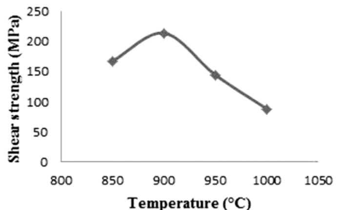
Fig. 5. Shear strength for diffusion brazed joints processed for 60 min
