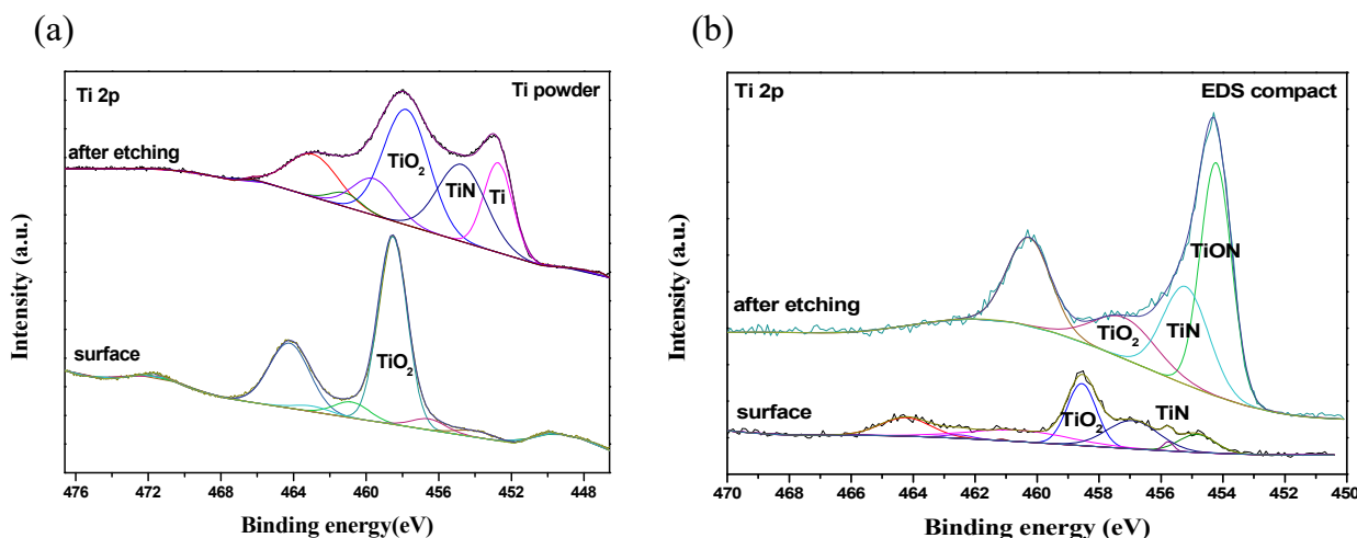
Fig. 4. XPS high resolution spectra of the Ti 2p region before and after \text{Ar}^+ etching of (a) as-received Ti powder and (b) compact discharged at 1.5 kJ of input energy
