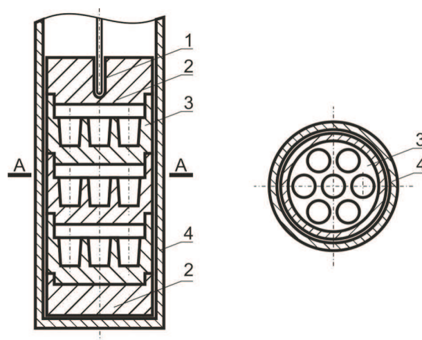
Fig. 1. Apparatus for the equilibrium saturation. (1 – [Ni-(Ni-Cr)] thermocouple and alumina sheath for thermocouple, 2 – graphite blocks, 3 – graphite blocks with grooves for alloys, 4 – chamber)
