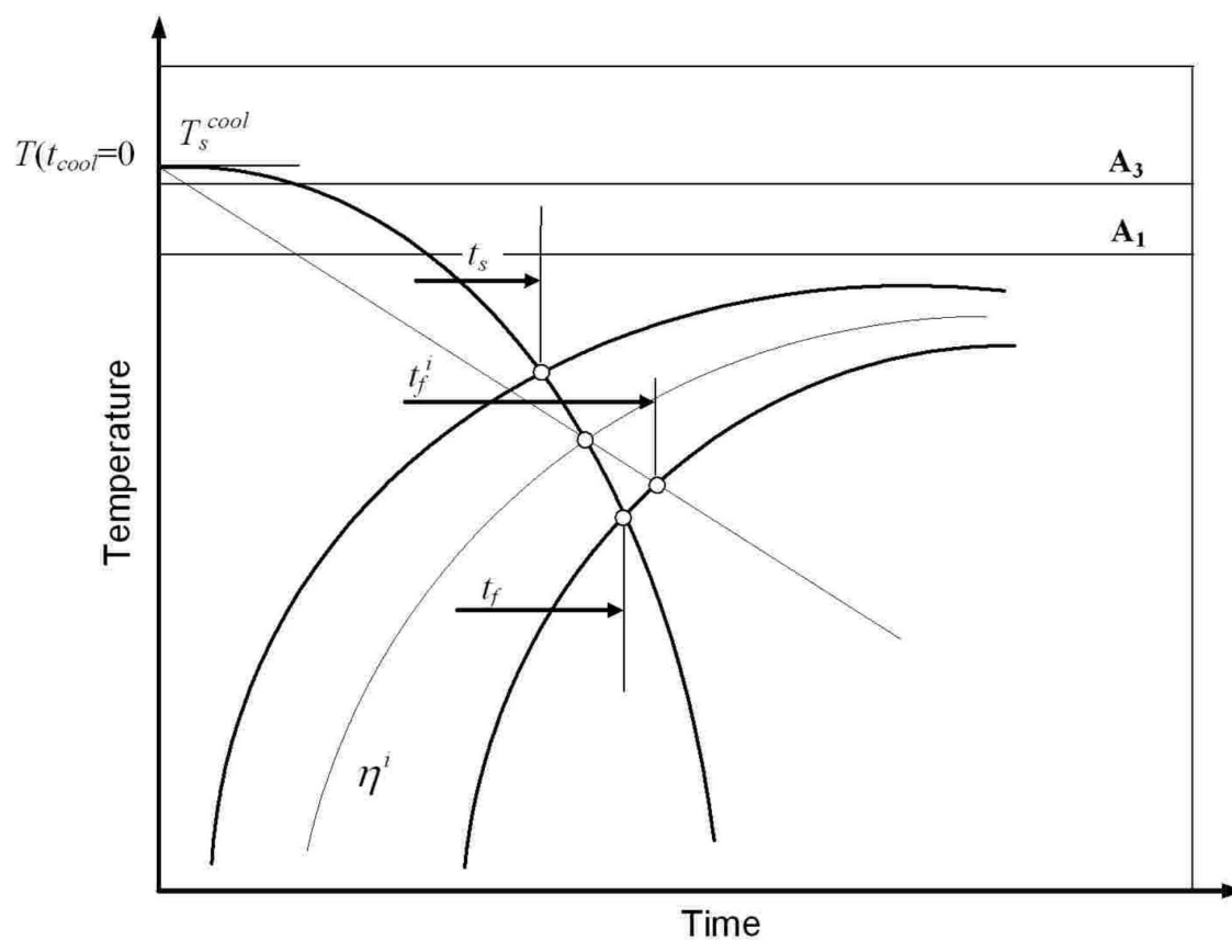
Fig. 3. Determination of time t_f in the parallel simulation (curve CCT, cooling)
