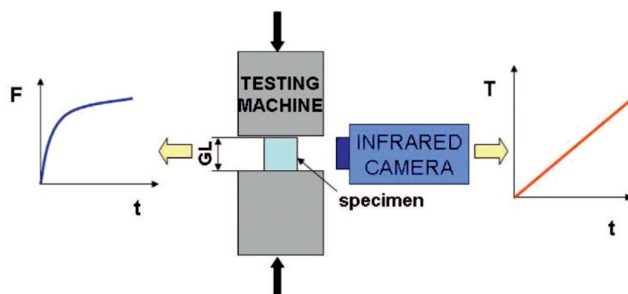
Fig. 1. Diagram and photograph of the experimental set up applied for investigation of mechanical and temperature characteristics of the FSMA loaded in compression test
