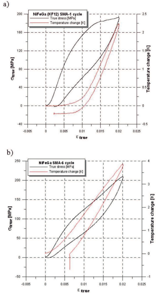
Fig. 4. Stress-strain and temperature-strain curves obtained for 1 st and 6 th cycles of compression polycrystalline NiFeGa with strain rate 10^{-2}s^{-1} and within the strain range 2%
