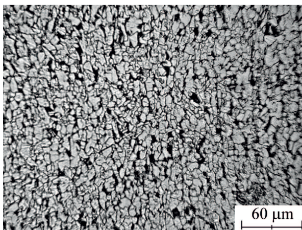
Fig. 9. The microstructure of the specimen after rolling simulation according to scheme 7 from Table 2
