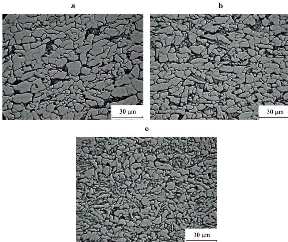
Fig. 10. The microstructure of the specimens after rolling simulation according to scheme 7 from Table 2 cooled after deformation at different rates: a – 3^{\circ}\text{C/s} , b – 30^{\circ}\text{C/s} , c – 50^{\circ}\text{C/s}
