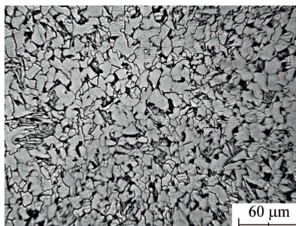
Fig. 7. The microstructure of the specimen after rolling simulation according to scheme 5 from Table 2
