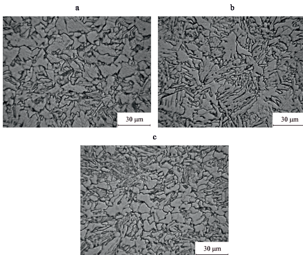
Fig. 12. The microstructure of the specimens after rolling simulation according to scheme 7 from Table 2 cooled immediately after deformation at the rate of 30°C/s to the temperature: a – 600°C, b – 500°C, c – 400°C, and then to the surrounding temperature at the rate of 1.5°C/s
