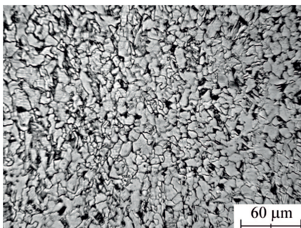
Fig. 8. The microstructure of the specimen after rolling simulation according to scheme 6 from Table 2
