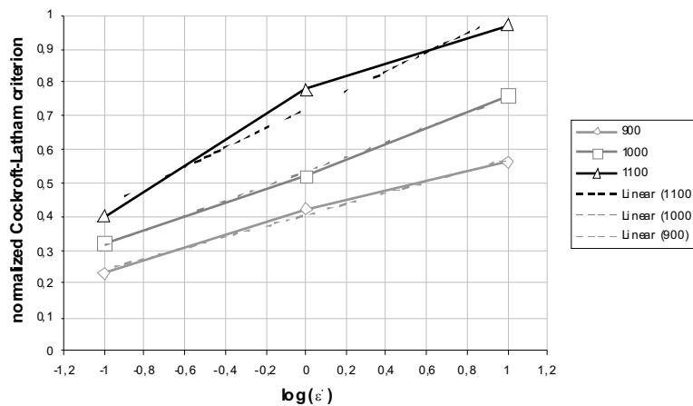
Fig. 4. Relationship of the normalized Cockroft – Latham criterion to the log (ε̇)
