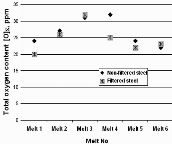
Fig. 6. [O]_T total oxygen content variation in each of the melt sequence (third trial) – SE03 steel
