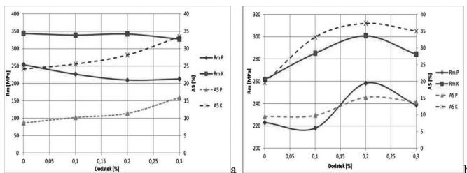
Fig. 3. Graphic representation of the CuSn10P(a) bronze and CuSn10Zn2(b) bronze; the samples cast into sand and metal moulds. Kupmod B modifier
