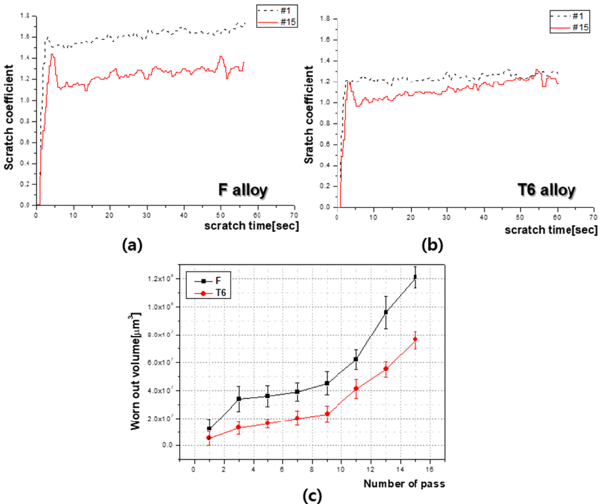
Fig. 4. Scratch wear properties with increasing number of pass (a) scratch coefficient of F alloy, (b) scratch coefficient of T6 alloy and (c) worn out volume
