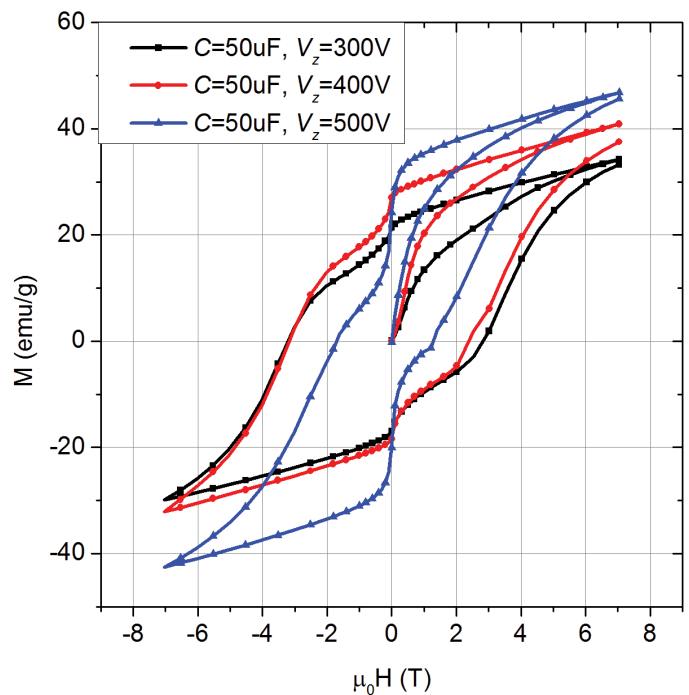
Fig. 3. Hysteresis loops for the samples sintered with C = 50 \mu\text{F} and different voltages
