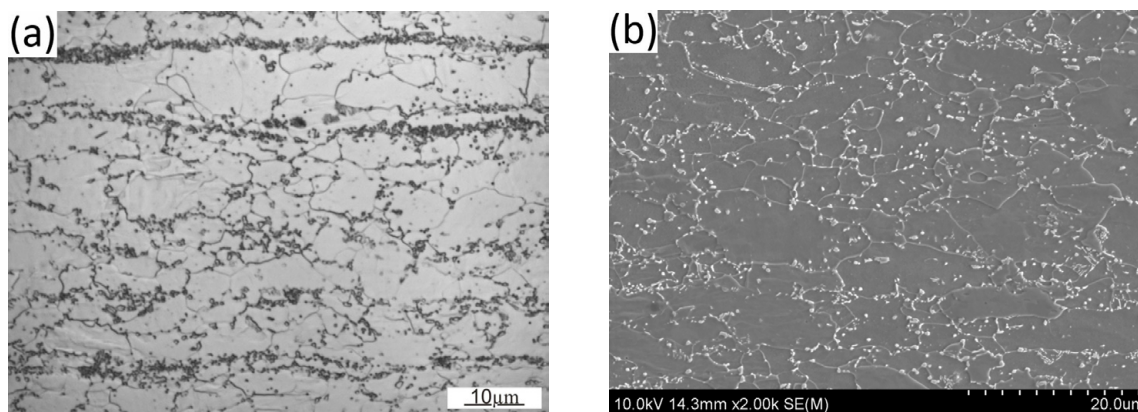
Fig. 1. Microstructure of steel sheet before deep drawing: (a) light microscopy; (b) scanning electron microscope (SEM), etched with 2 % nital
