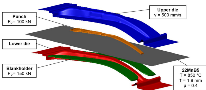
Fig. 5. Tools assembly and process parameters applied in the numerical simulation using Pam-Stamp 2G software
