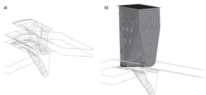
Fig. 1. Model of die: a) with rigid tools, b) with elastomeric tools
