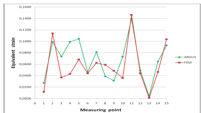
Fig. 9. The distribution of strain at the measuring points drawpiece designated Argus and FEM method
