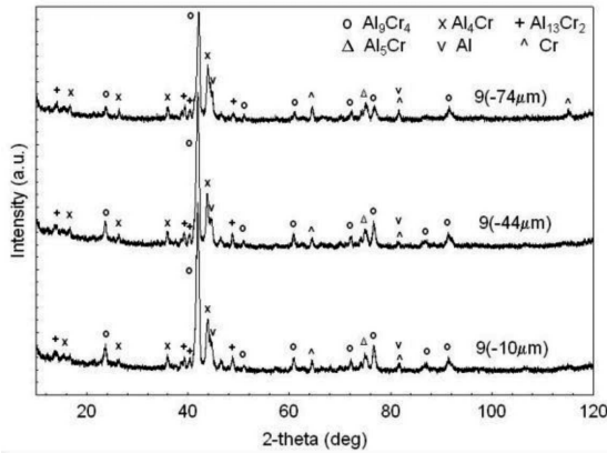
Fig. 3. XRD patterns of 9Al + 4Cr combustion products. The granularity of Cr powder (-10, -44 and -74 \mu\text{m} ) induces relatively small changes in the product phase composition
