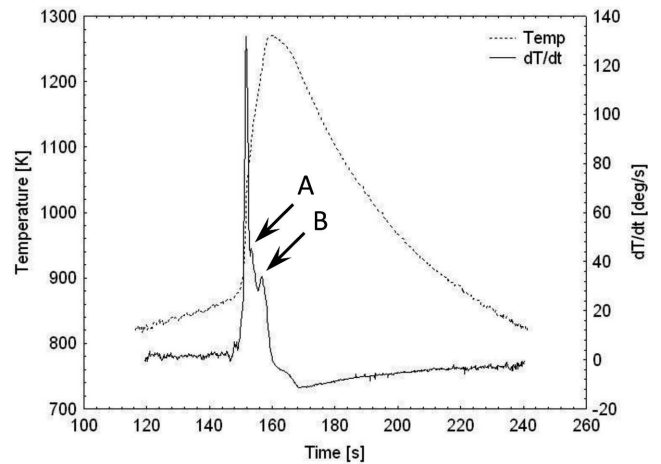
Fig. 1. Temperature profile and its differential for samples with granularity of Cr particles -44\mu\text{m} . Phase transformations are: \text{L} + \text{Al}_7\text{Cr} \rightarrow \text{L} + \text{Al}_{11}\text{Cr}_2 at A and \text{L} + \text{Al}_{11}\text{Cr}_2 \rightarrow \text{L} + \text{Al}_4\text{Cr} at B
