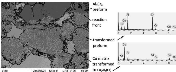
Fig. 4. The front of reactive infiltration of \text{Al}_9\text{Cr}_4 preform with Cu. EDS analysis of the transformed phase composition for preform and Cu matrix
