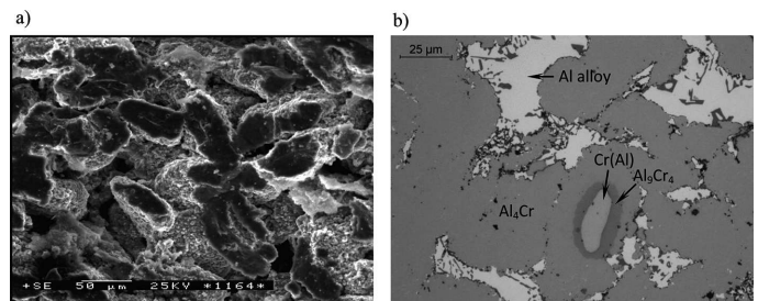
Fig. 2. Fracture of a preform produced from the mixture of 4\text{Al} + \text{Cr}(-74\mu\text{m}) powders (a), cast composite material obtained by infiltration of the preform with aluminum alloy (light background)
