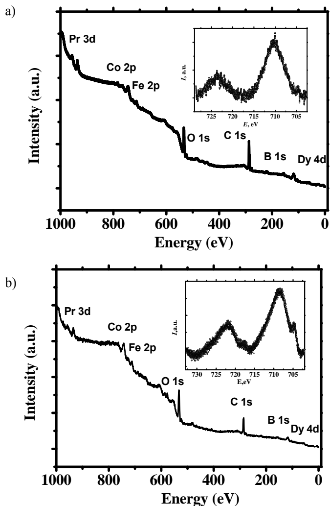
Fig. 3. Survey XPS spectrum of the surface of sample 2 at 300 K: (a) before and (b) after annealing. Core level spectra of the Fe 2p level are shown in inserts
