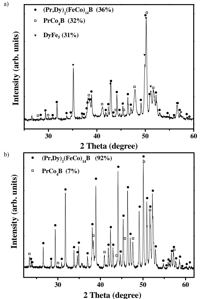
Fig. 2. Survey X-ray diffraction spectra for sample 2 before (a) and after (b) annealing at 900°C
