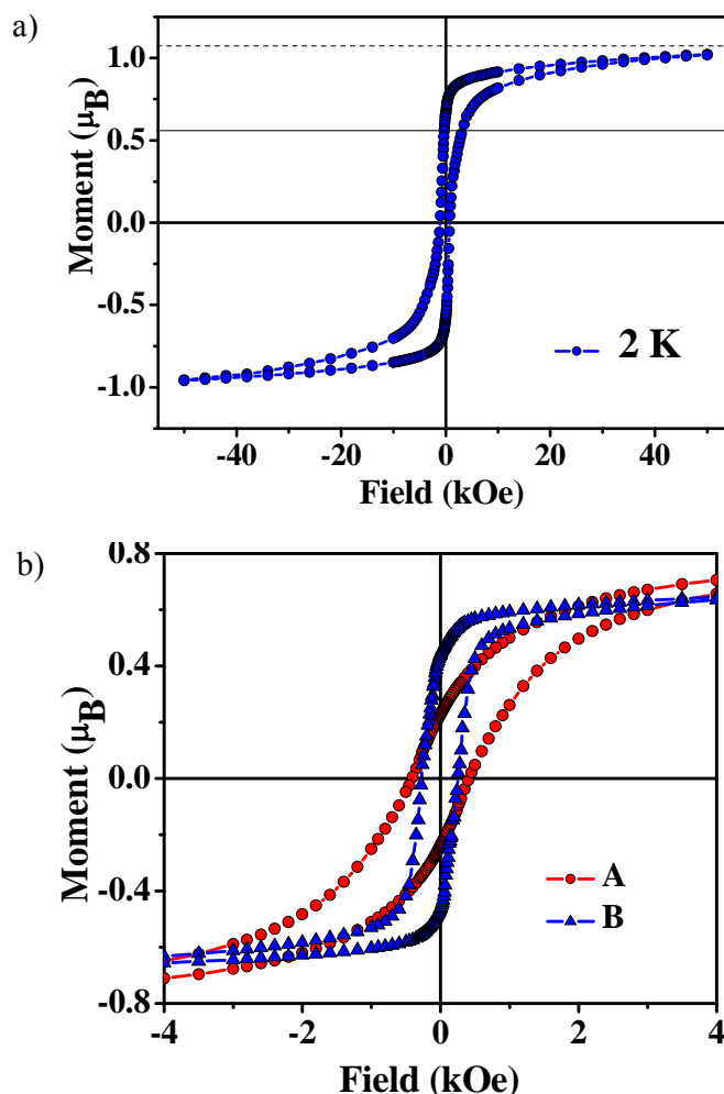
Fig. 4. Magnetic hysteresis of sample 2: (a) at T = 2 K before annealing, (b) at 300 K before annealing (circles) and after annealing (triangles). Calculated \mu_{\text{eff}} value for bulk and surface atomic concentrations are shown by dashed and solid horizontal lines, respectively.
