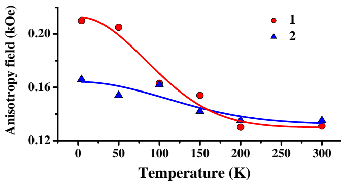
Fig. 8. Temperature dependence of anisotropy field H_A in the samples (1) (Pr 0.70 Dy 0.30 ) 15.3 (Fe 0.48 Co 0.52 ) 70.7 B 14.0 , (2) (Pr 0.85 Dy 0.15 ) 16.5 (Fe 0.17 Co 0.83 ) 69.4 B 14.1 . Solid lines are approximations described in the text
