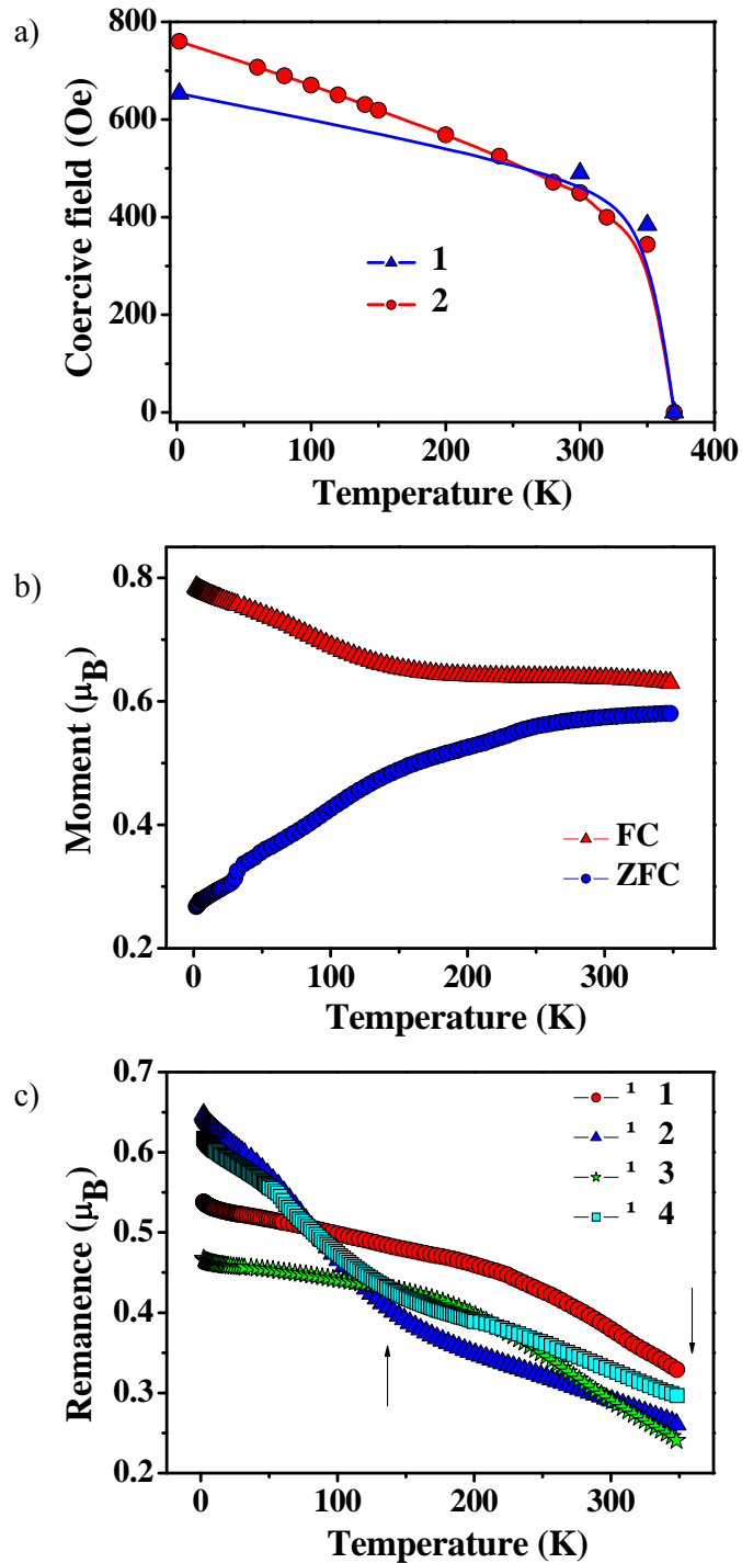
Fig. 5. Temperature dependencies of: (a) coercive force H_c of samples 1 and 2, (b) magnetization M of sample 2 cooled in 10 kOe magnetic field (FC, triangles) and zero magnetic field (ZFC, circles). Measurements were performed in 1 kOe magnetic field, (c) remnant magnetization M_{\text{rem}} of samples 1-4 after cooling down to 2 K in 50 kOe magnetic field (numeration of the curves corresponds to that of the samples)
