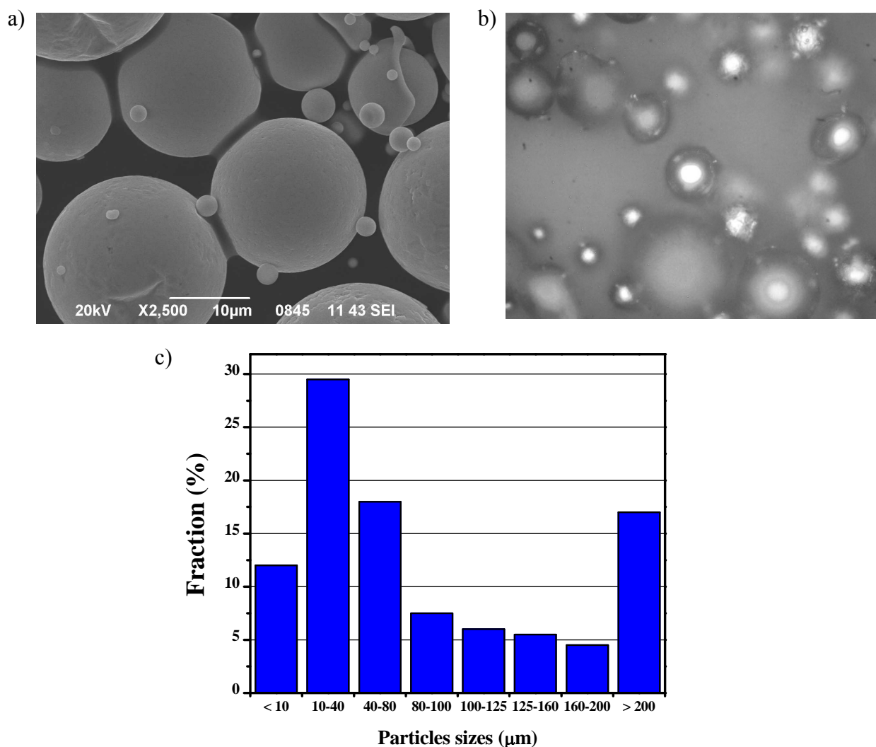
Fig. 1. SEM image of microparticles in “as grown” sample 2 (a), optical microscopy image (b), and size distribution of particles in sample 2 (c)
