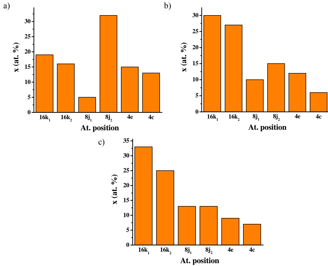
Fig. 7. Populations of the atomic sites in the TM sublattice by Fe atoms in series of the samples with progressively increased Fe content: (a) Pr 2 (Fe 0.17 Co 0.83 ) 14 B, (b) (Pr 0.68 Dy 0.32 ) 2 (Fe 0.53 Co 0.47 ) 14 B, (c) (Pr 0.39 Dy 0.41 Gd 0.20 ) 2 (Fe 0.69 Co 0.31 ) 14 B
