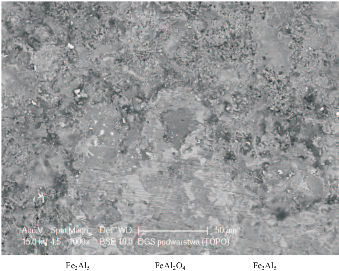
Fig. 5. Surface topography of DGS FeAl coating after grinding by 50 \mu\text{m}
