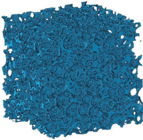
Fig. 6. Finite element model of ceramic foam (4×4×4 mm) created by using element of size A
