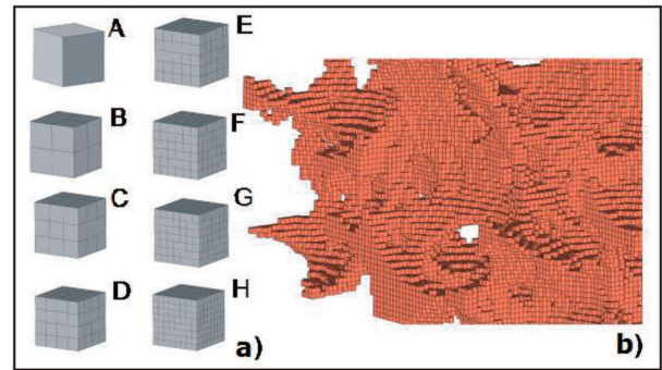
Fig. 3. (a) The finite elements based on different number of voxels, the elements A, B, ..., H represent 1^3 , 2^3 , ..., 8^3 voxels respectively, (b) the part of view for generated finite element mesh with element size A
