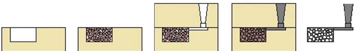
Fig. 2. The principle of the liquid metal infiltration into the mould cavity filled with precursors, from the left: the mould, the mould cavity filled with precursors, the assembled mould, metal casting into the mould cavity, a metal foam casting after removal of precursors
