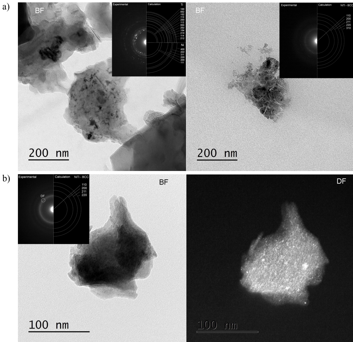
Fig. 4. TEM images (bright field – BF and dark field – DF) as well as SAED patterns observed for the powders milled after 20 hrs (a) and 100 hrs (b)
