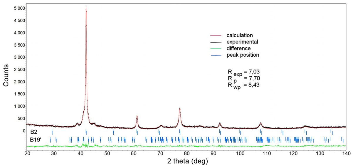
Fig. 8. Results of the Rietveld refinement for NiTi alloy after crystallization at 600°C
