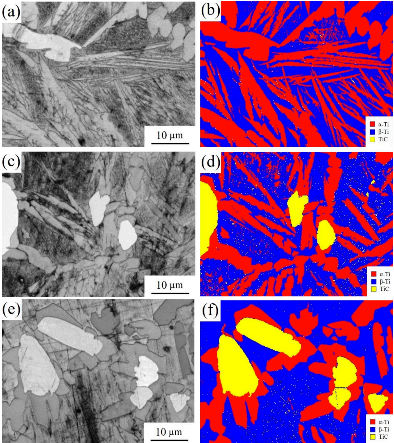
Fig. 7. The EBSD analysis for various mass% \text{Mo}_2\text{C} added to Ti-8Nb-4Co alloys after sintering at 1300^\circ\text{C} for 1 h: (a), (c), (e) image quality, (b), (d) and (f) phase mapping, which are 1 \text{Mo}_2\text{C} , 3 \text{Mo}_2\text{C} and 5 \text{Mo}_2\text{C} , respectively
