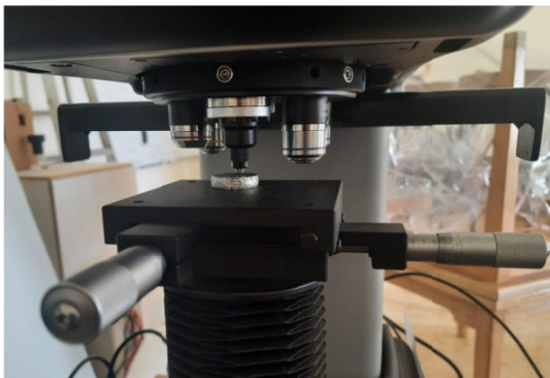
Fig. 5. Microhardness tester
