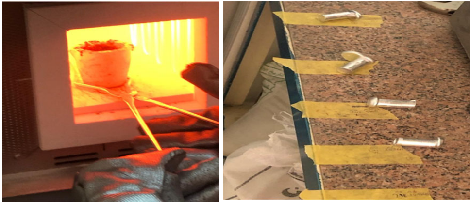
Fig. 2. Casting of Al-Cu alloys process
