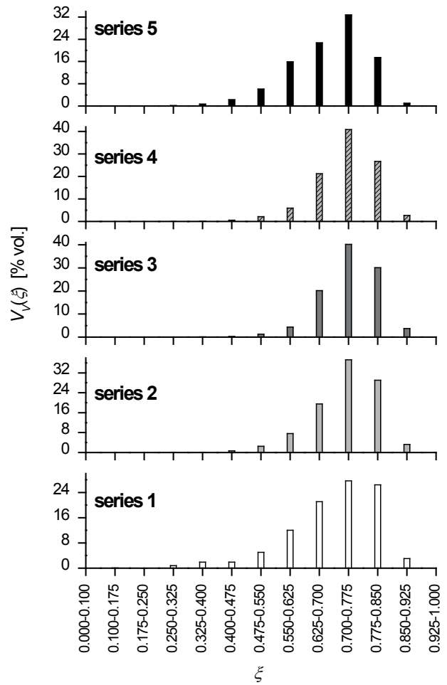
Fig. 4. A volume fraction of the grains with the \xi shape index
