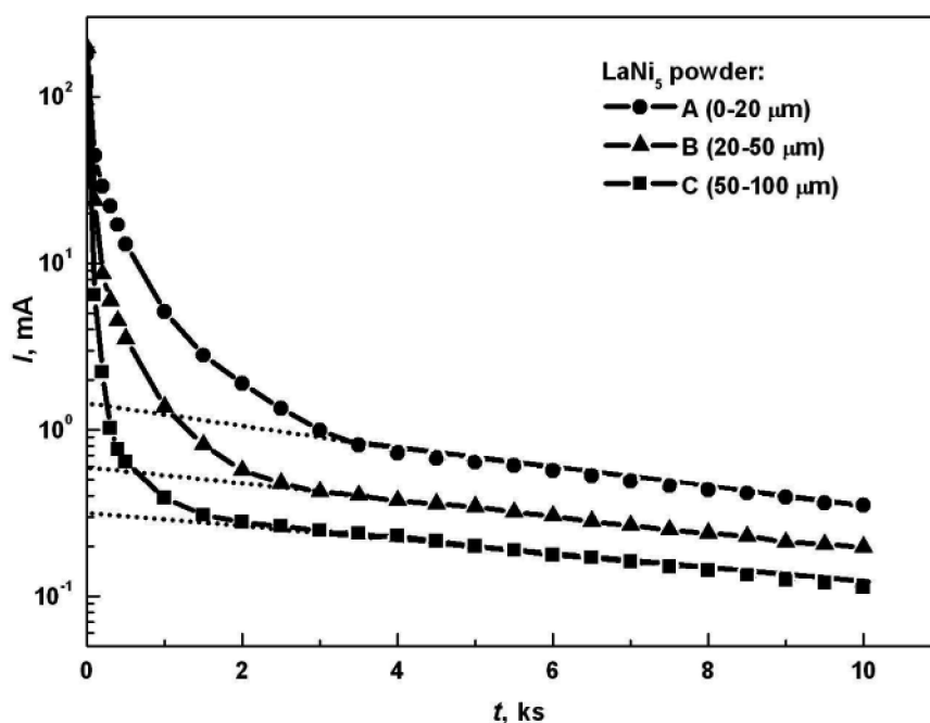
Fig. 2. Chronoamperometric curves for three composite electrodes (made of A, B and C \text{LaNi}_5 powders) at constant discharge potential, E = -0,3 V (6 M KOH, 25^\circ\text{C} , Ar)
