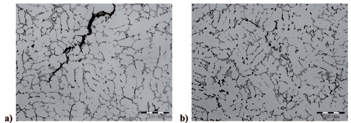
Fig. 1. Microstructure of casting with not acceptable defect (a) and acceptable casting (b) of AlSi5Cu3 alloy
