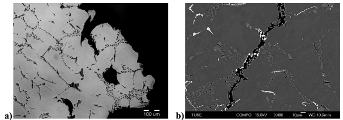
Fig. 2. Character of crack propagation in structure of casting with not acceptable defect documented by LM (a) and SEM (b)
