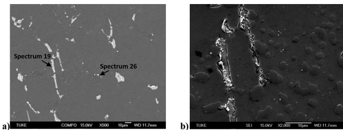
Fig. 4. Morphology of intermetallic phase particles in structure of suitable casting (a) and detail of particles (b)
