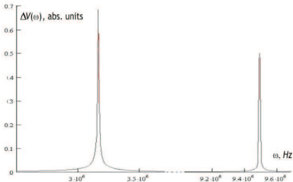
Fig. 3. The dependence of the photoacoustic signal amplitude on the Bessel light beam amplitude modulation frequency
