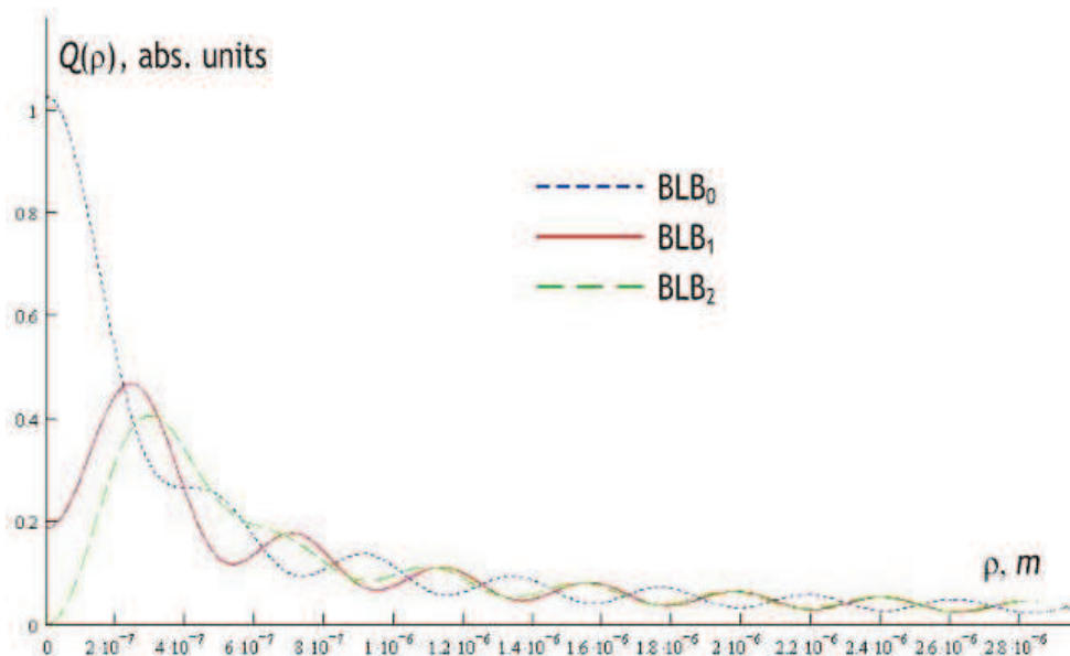
Fig. 2. The dependence of the Bessel light beam energy dissipation on the radial coordinate and the mode of radiation
