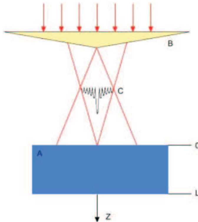
Fig. 1. Scheme of photoacoustic signal registration: A – piezoelectric sample, B – axicon, C – Bessel light beam
