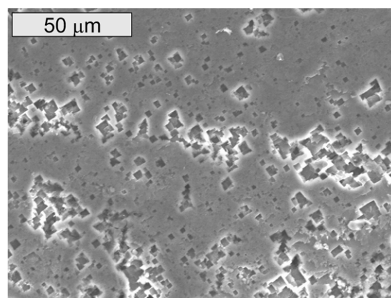
Fig. 1. A general view of a "crystallographic attack" observed in the solid solution of aluminium alloy AW7075 [unpublished own materials]
