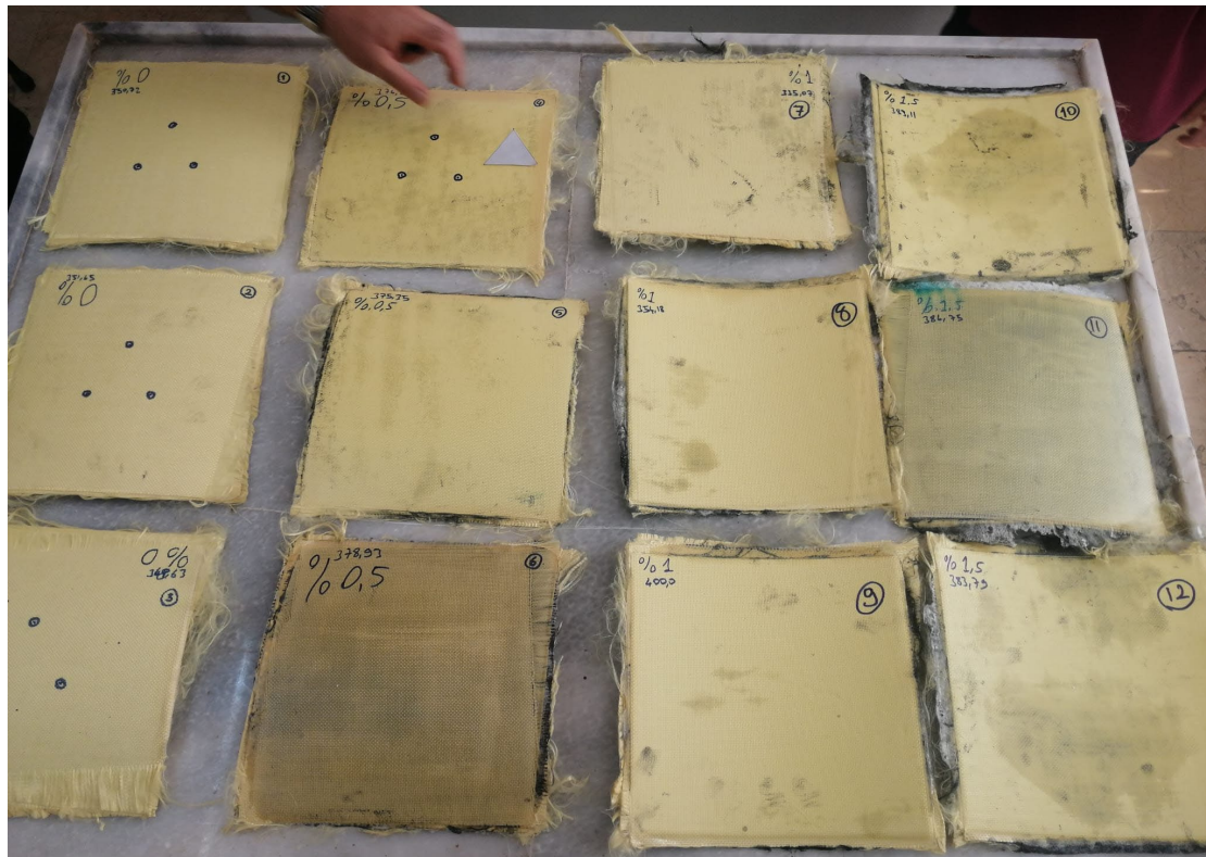
Fig. 5. Ballistic plates
