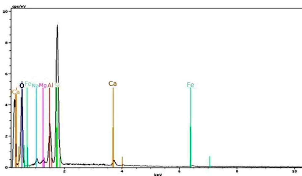
Fig. 2. Nanoclay Element Composition
