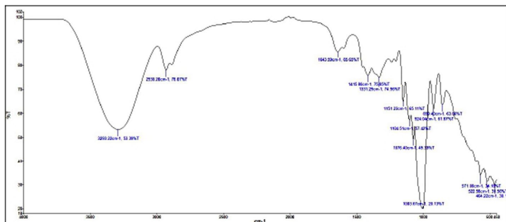
Fig. 3. NPF's FT-IR analysis result
