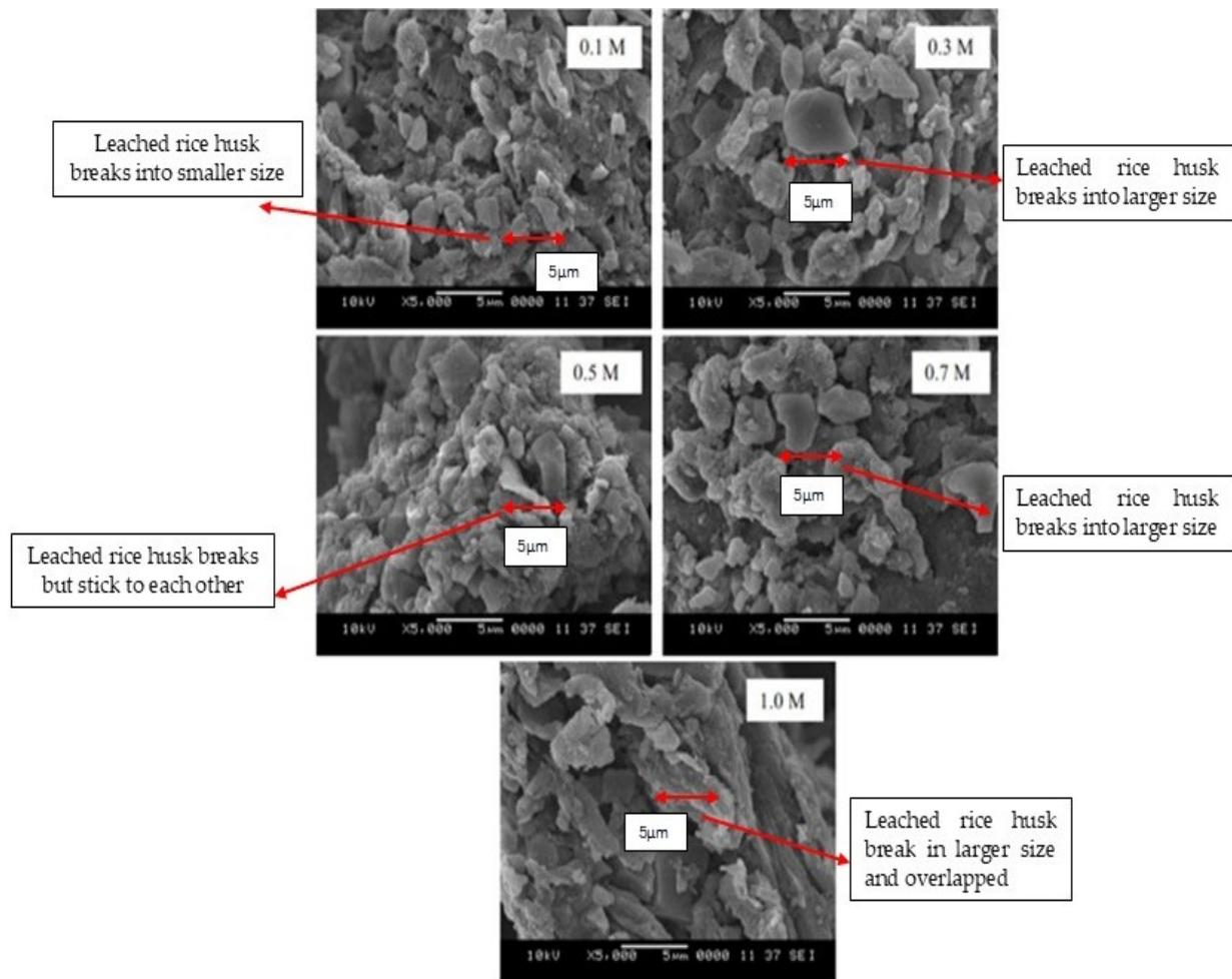
Fig. 4. Microstructure images of magnified leached rice husk at various concentrations of citric acid
